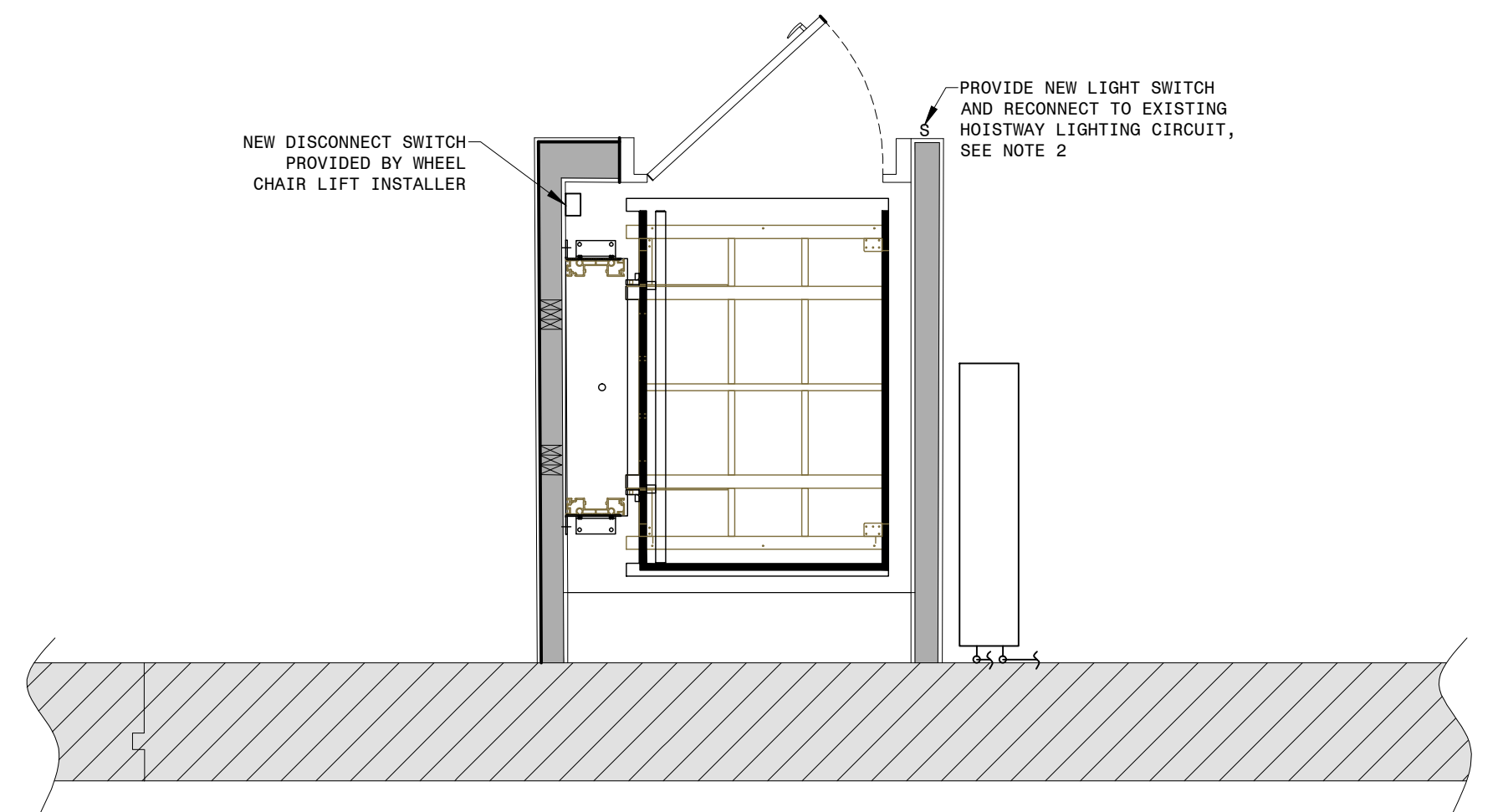
BASEMENT PLAN 1/2"=1'-0"
