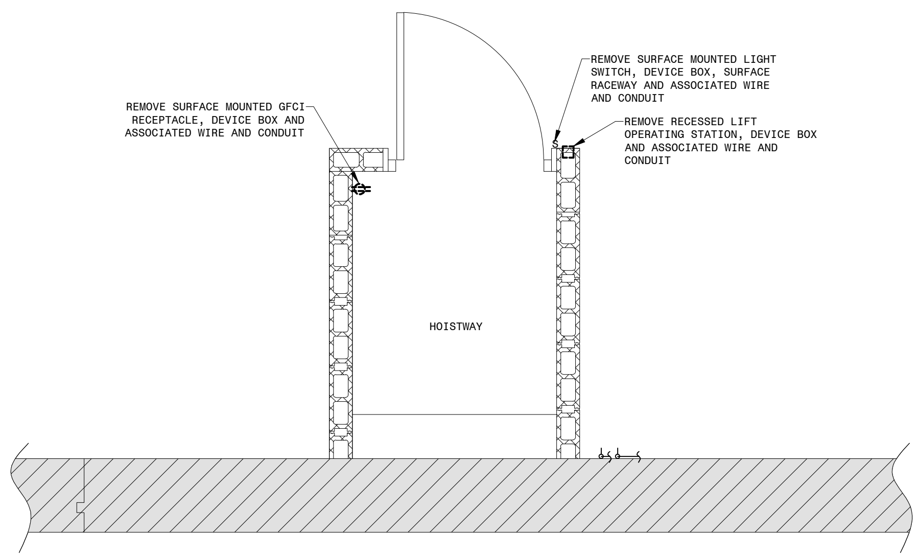
BASEMENT DEMOLITION PLAN 1/2"=1'-0"
