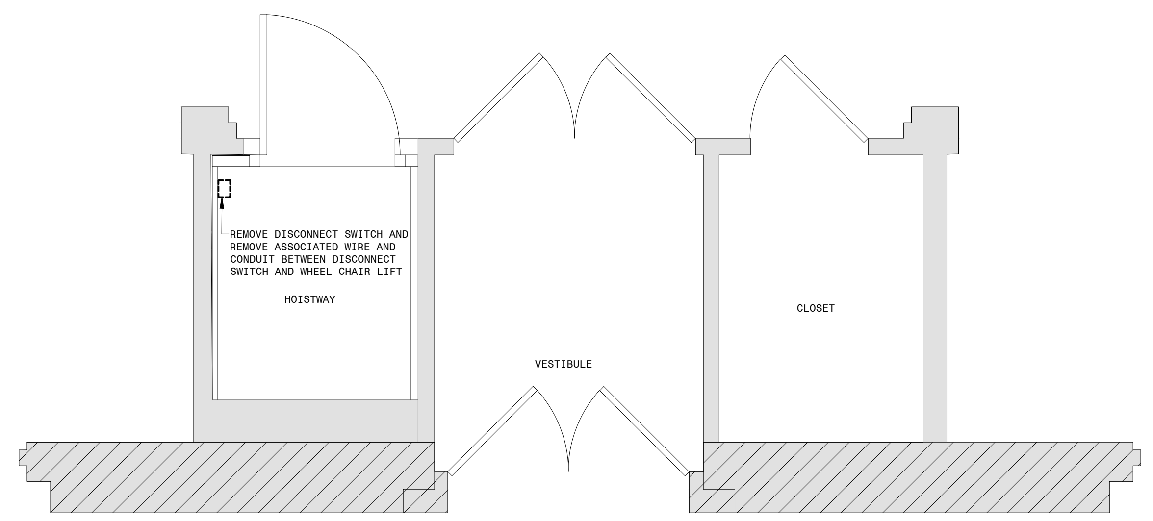
FIRST FLOOR DEMOLITION PLAN 1/2"=1'-0"
